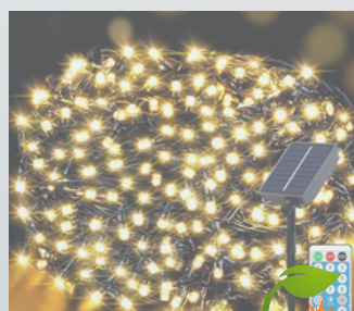
FL-15-SOL 10W LED Solar Fairy Light, Super Bright LED's, 15meter, 220VAC, IP44, Warm White
