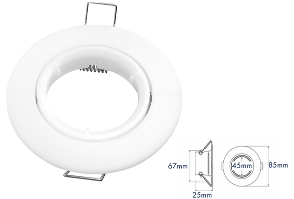
OL-912-W ADJUSTABLE ROUND DOWNLIGHT FITTING ONLY WITH REMOVABLE RETAINING RING
