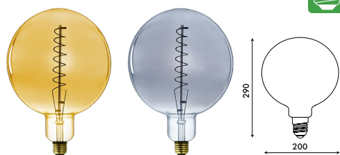
OL-G200-4W-D- 4W LED E27 FILAMENT BULB
