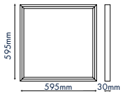
EBL-LED600-3CCT 600X600 BACKLIT LED PANEL LIGHT
